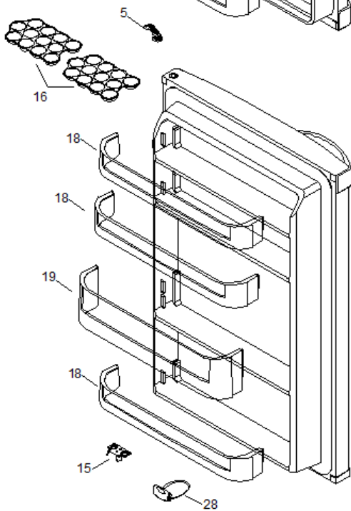
9 PUERTA REFRIGARADOR ENS. COMPL. DOOR FF ASM.
